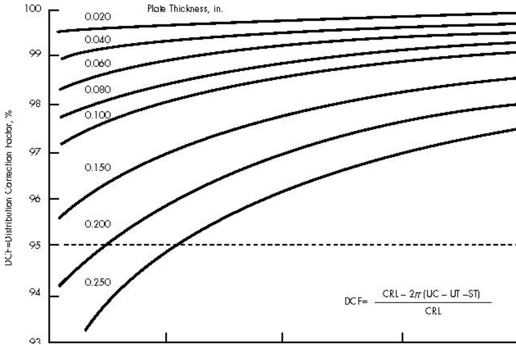
Figure 2: Distortion Correction Factor – MacDermid Liquid Photopolymer Plates
